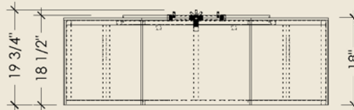
FRONT ELEVATION
